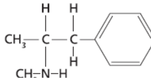
Desoxyephedrine l-methamphetamine
