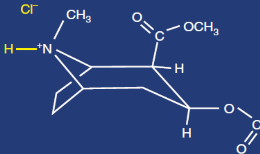
Cocaine Hydrochloride
