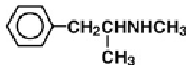
Methamphetamine
