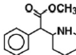
Methylphenidate
