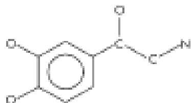
norepinephrine
